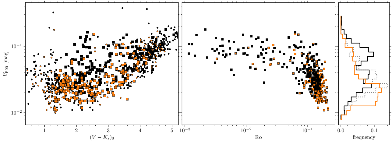
Figure 5.2: Left: V band variability amplitude ( V_{P90} ) for stars in NGC 3532 (orange), compared with those of the zero-age main sequence open cluster NGC 2516 (black) for both rotators (squares) and non-rotators (circles). Stars in NGC 3532 generally have lower variability. Centre: V_{P90} against Rossby number Ro for the rotators in NGC 3532 and NGC 2516. The distribution can be seen to resemble the activity-rotation relation previously known from chromospheric and coronal activity, and shows that the photospheric activity amplitude has a similar structure. Right: Histogram of the variability amplitudes for the members of the two open clusters showing that the high amplitude stars of NGC 3532 are much reduced in comparison with NGC 2516. The grey histogram is restricted to NGC 2516 stars with (V - K_s)_0 < 4 and confirms that the high-amplitude peak in NGC 2516 is mostly attributed to the fast rotating M dwarf members, a population absent in our NGC 3532 data.
