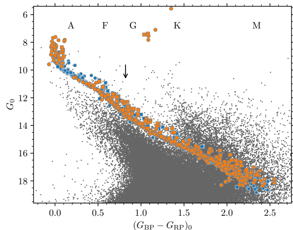
Figure 4.3: Colour-magnitude diagram in Gaia DR2 colour for NGC 3532 with cluster members highlighted. Radial velocity members from Fritzewski et al. 2019 are marked in orange and additional proper motion members in blue. The enormous field star population is shown in grey in the background. All data are dereddened with the average reddening value towards NGC 3532 ( E_{G_{BP}-G_{RP}} = 0.046 ). Likely binaries are marked with squares. At the top, we indicate the different spectral types from Pecaut & Mamajek 2013 for orientation. The arrow indicates the Solar colour (Casagrande & Vandenberg 2018). For colour-magnitude diagrams in other colours see Fig. 4.5 below and Fig. 14 of F19.
