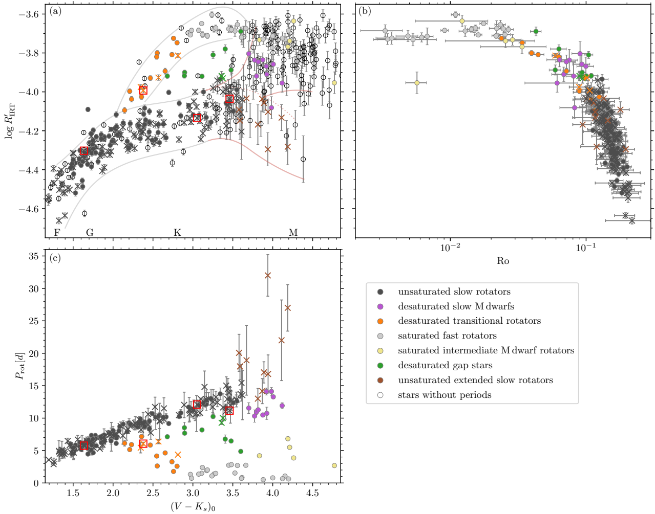
Figure 5.6: Same as Fig. 5.4 but now including the newly identified (activity-informed) rotation periods (crosses). Each new period is also colour-coded to match the previously determined rotational groups, enabling cross-identification as in Fig. 5.4. This diagram includes the unsaturated extended slow rotator sequence (brown), absent in Fig. 5.4. The light curves and periodograms of the four stars marked with red squares (both in the CAD and CPD) are displayed in the Appendix Fig. 5.9 to demonstrate the viability of deriving these activity-informed periods.
