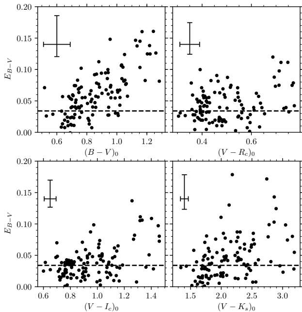
Figure 2.15: Reddening estimate calculated from the effective temperatures and the measured colours. For each intrinsic colour the reddening was calculated and converted to E_{B-V} with the coefficients from Johnson 1968. The dashed line marks the finally adopted reddening E_{B-V} = 0.034 mag. In the upper left of each panel we show the typical uncertainties.
