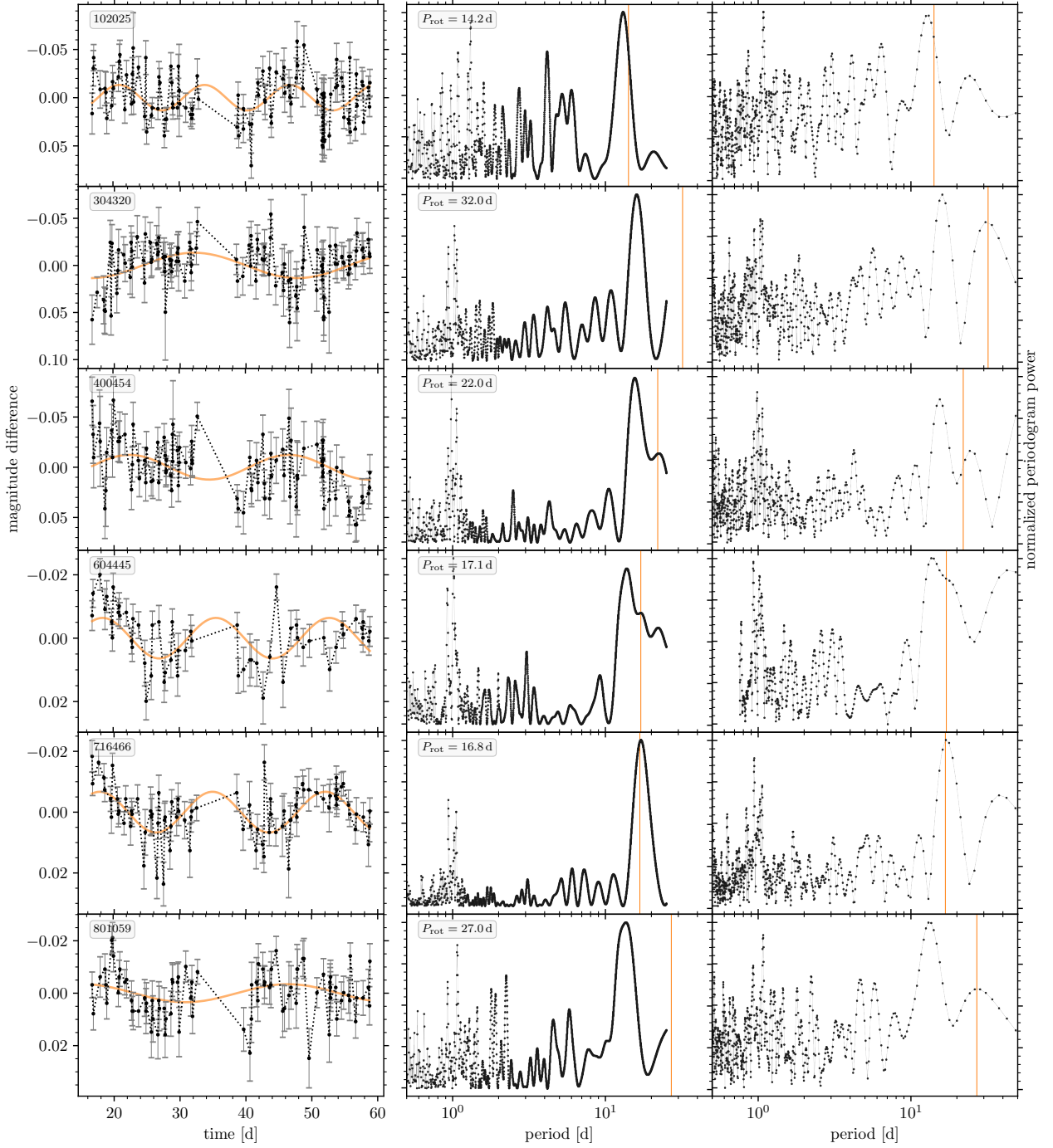
Figure 5.8: Left column: Light curves for the early M dwarfs of low stellar activity in NGC 3532 that have newly-identified rotation periods. The orange line is a sine fit to the data with the newly-identified likely rotation period. The first two light curves (from top) are from V 120 s exposures while all other are from I_c 600 s images. Centre column: Corresponding normalized generalized Lomb-Scargle diagram with the selected rotation period marked by the vertical line. Right column: Same as centre column but with the CLEAN periodogram. The offset between the peaks and the position of the best period for 102025 in the first row is due to the different peak positions in the phase-dispersion minimization and Gregory-Loredo periodograms (not displayed).
