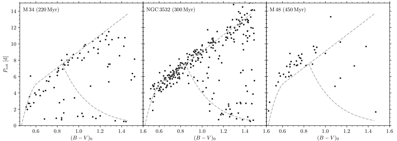
Figure 4.9: Colour-period diagrams for M 34 (Meibom et al. 2011), NGC 3532 (this work), and M 48 (Barnes et al. 2015) (from left to right) showing the period evolution in this 220 – 450 Myr age range. Fiducial lines for NGC 3532 (dashed) are reproduced in the panels for M 34 and M 48. We see that the M 34 rotation period distribution is mostly below the NGC 3532 fiducials while the M 48 distribution is above them. This informs us that M 34 is younger than NGC 3532 while M 48 is older.
