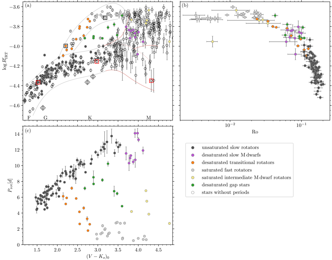
Figure 5.4: Interconnection between chromospheric activity, rotation, and mass. The colour-activity diagram, (a), connects the rotation-activity diagram (b) with the colour-period diagram (c). Top left: Chromospheric emission ratio \log R'_{\text{IRT}} against intrinsic (V - K_s)_0 colour for members of NGC 3532. Member stars with measured rotation periods are shown with filled circles and those without photometric rotation periods with open circles. The majority of the data points delineate very clear sequences, indicating the cohesion of chromospheric activity evolution within the coeval stars of an open cluster. The colour coding of the different groups is indicated in the legend on the lower right and is the same in all three panels. The thin lines indicate the sequences described in the text. The stars emboxed in red and black squares are the low-activity and high activity stars respectively shown in Fig. 5.1 (top to bottom in Fig. 5.1 corresponds to left to right in this figure). The bluest of these stars has roughly the Solar colour. Stars marked by diamonds are outliers (discussed in the text). Top right: Corresponding rotation-activity diagram, showing the chromospheric emission ratio against the Rossby number Ro . The rotation-activity diagram is remarkably clean, despite the diversity in chromospheric activity. Bottom left: Colour-period diagram of NGC 3532 with groups of stars distinguished by colour. This diagram is nearly a mirror image of the colour-activity diagram, with higher-activity stars being clearly mapped one-to-one onto the faster rotators.
