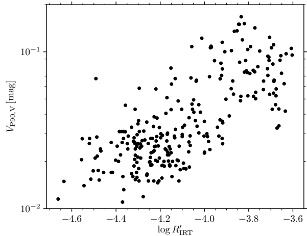
Figure 5.3: Photometric variability amplitude in the V band V_{P90,V} against chromospheric emission ratio \log R'_{\text{IRT}} . The two activity indicators are correlated and represent two facets of the underlying magnetic activity.
