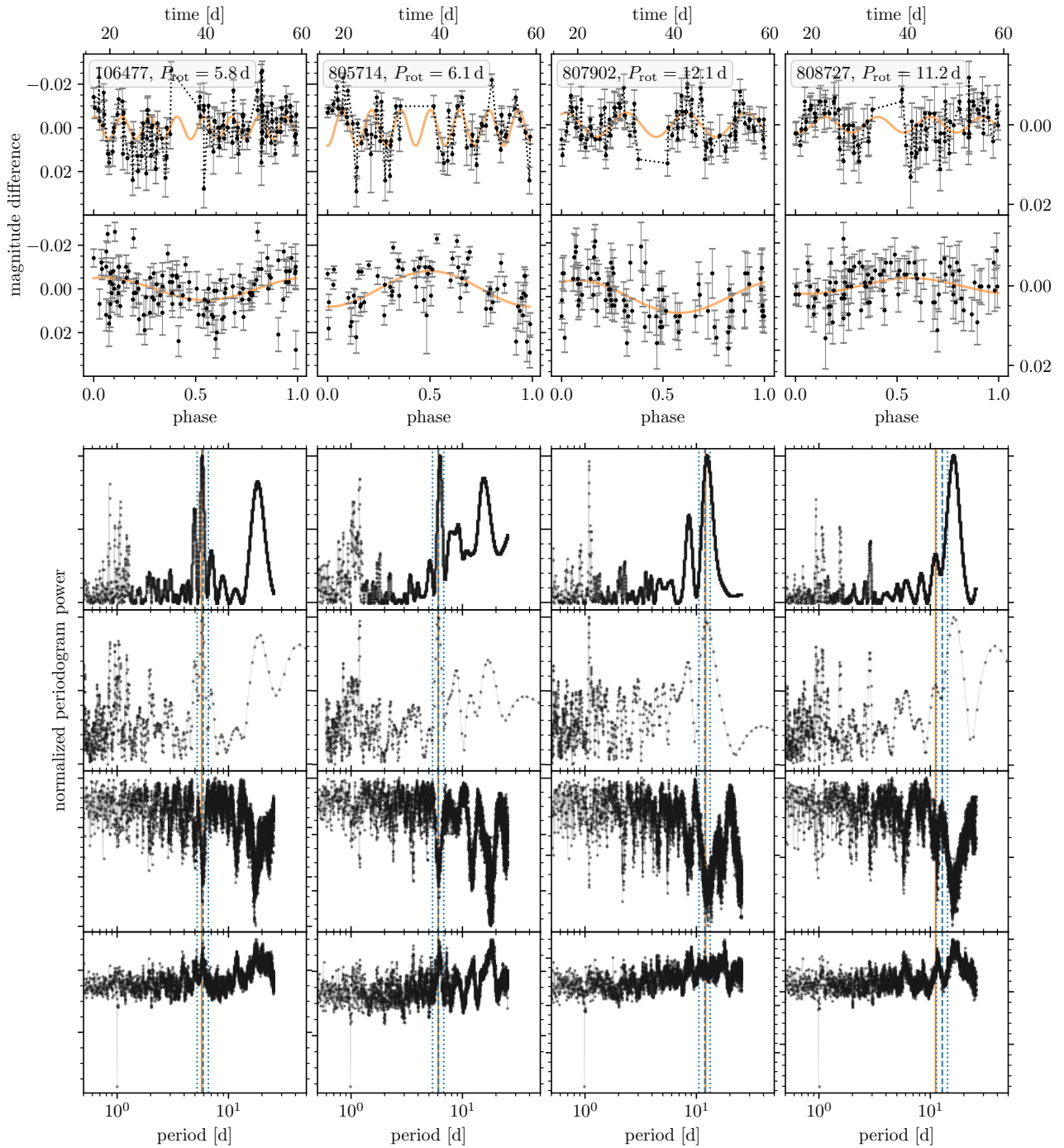
Figure 5.9: Four examples of light curves and their associated periodograms for (non-M) stars with newly-identified, activity-informed rotation periods. Each column shows the data of one star. The two upper panels show the light curves in both the time and phase domains. We fit a sine with the rotation period and display it along with the data. The left scale is valid for the two left-most plots, while the right scale is for the two light curves on the right. The lower panels show, from top to bottom, the Lomb-Scargle, CLEAN, phase-dispersion minimization, and Gregory-Loredo periodograms. In each periodogram, we mark both the rotation period (orange line) and the period estimated from the activity and its uncertainty (blue lines). Unlike the other periodograms, in the phase-dispersion minimization the best periods are represented by dips.
