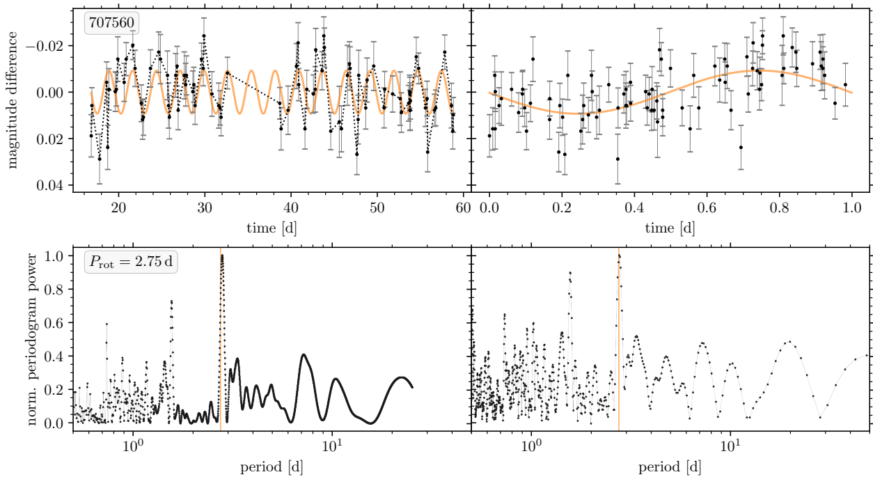
Figure 5.7: Light curve in time ( top left ) and phase space ( top right ) as well as the Lomb-Scargle periodogram ( bottom left ), and CLEAN periodogram ( bottom right ) for the outlier (707560) in the rotation-activity diagram.
