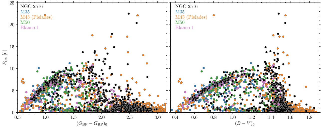
Figure 3.17: Representative ZAMS rotation period distribution shown in combined colour-period diagrams of all considered open clusters in both Gaia (G_{BP} - G_{RP})_0 (left) and (B - V)_0 colours (right). The fast and slow sequences, including the extended slow rotator sequence are evident, as is the less-densely occupied region between the sequences. The display colours of the individual open clusters are the same as in Fig. 3.16, and Fig. 3.23 provides separate comparison panels for the individual clusters in B - V colour. See Fig. 3.24 for an approximate way to represent this distribution in a colour-independent way using elementary functions of the convective turnover timescale.
