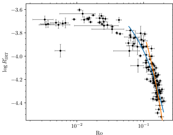
Figure 5.5: Rotation-activity diagram with two possible fits to two regions of interest: all unsaturated stars (blue, Ro > 0.06 ) and only the slow rotators (orange, Ro > 0.11 ).
