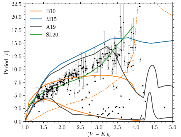
Figure 4.8: Comparison between the NGC 3532 rotation periods and 300 Myr stellar rotation models. In orange, we show both the slow and fast rotator model from Barnes 2010. The dashed line indicates the position of the rotational gap from B10. The asymptotic spin rate from Matt et al. 2015 for 300 Myr is shown in blue and the isochrones from Amard et al. 2019 for both the fast and slow rotators are given in grey, while the slow rotator isochrone from Spada & Lanzafame 2020 is shown in green.
