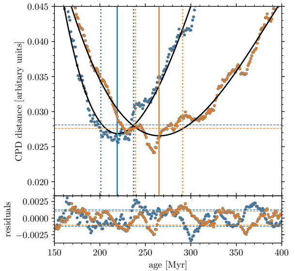
Figure 4.11: Rotational age for NGC 3532 with respect to the M15 (blue) and B10 (orange) models using the NGC 2516 rotation period observations as the starting point at 150 Myr. Top: Median distance between the slow rotator sequence of NGC 3532 and the evolved sequence of NGC 2516 against age. Coloured points show the measured distance and the solid black lines are the fitted polynomials. Their minima (219 Myr and 265 Myr) are marked by the solid vertical lines. The age uncertainties (18 Myr and 26 Myr) are indicated by the vertical dotted lines. The dashed horizontal line for each model marks the sum of minimum of the polynomial and the standard deviation of the residuals to illustrate the calculation of the age uncertainty. Bottom: Residuals of the fits with their standard deviations are marked using dashed lines.
