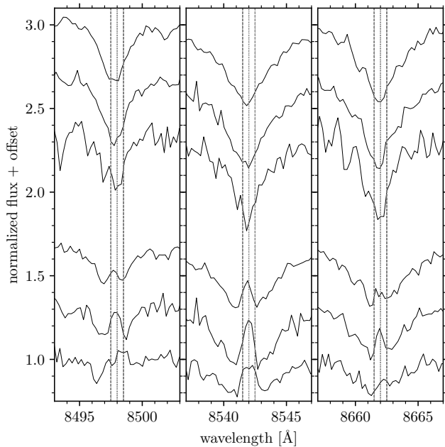
Figure 5.1: Spectral cut-outs for example stars of different chromospheric activity. The panels are each centred on one IRT line and shifted to the rest frame. The line centre is marked with a dotted line and the limits of the 1 Å-wide integration window with dashed lines. The spectra are grouped into low activity ( top ) and high activity stars ( bottom ). The latter feature prominent fill-ins of the line cores. Earlier spectral types are higher. The top most spectrum is from a G2 star, while the lowest is from an M3 star. All six stars are marked with squares in the colour-activity diagram in Fig. 5.4a.
