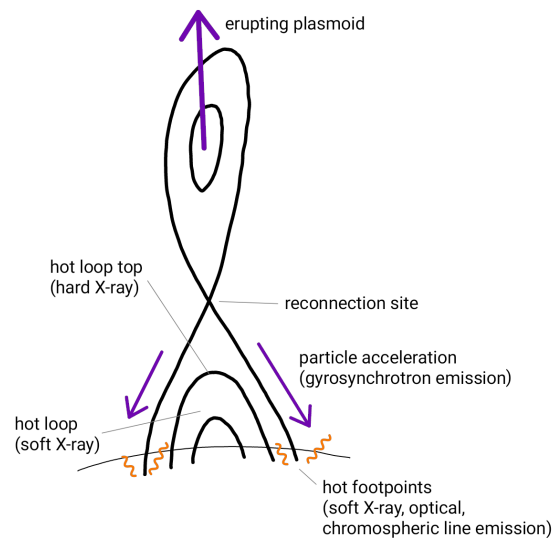
Figure 2.2: Simplified sketch of a flare loop (black lines) after re-connection. The magenta arrows indicate particles accelerated up- and downwards from the re-connection site in the corona.
