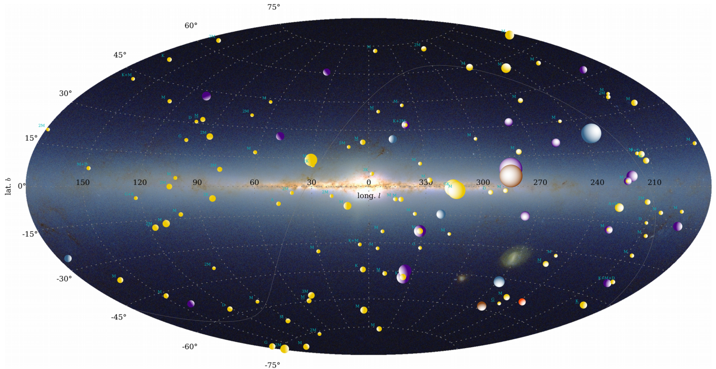
Fig. 1: Distribution of the known nearby ( d < 6.5 pc) stars and brown dwarfs (depicted as spheres) over the 2MASS near-infrared sky (Aitoff projection, galactic coordinates). These objects span masses of 2.0-0.075 and \sim 0.075 -0.007 Msol, respectively. The spheres are illuminated by a virtual source 25 pc ahead of the Sun and from the direction of rotation of the Galaxy ( l = 90 deg). Their size is proportional to their parallax (stars are shown half the size of brown dwarfs). Brown dwarfs of M-, L-, T-, and Y spectral types are indicated by red, brown, magenta, and blue colors, respectively. Stars are shown in yellow and annotated with their spectral types (underdashed annotations indicate known exoplanets). The Earth equator projected on the sky is represented by the gray curve.
